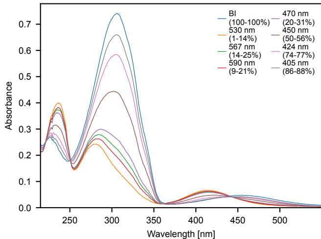
example_data/data_photoswitch-ABF440.xlsx
