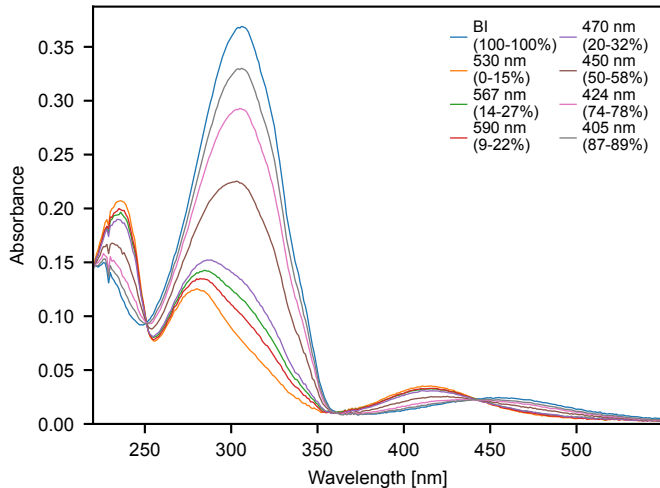
example_data/data_photoswitch-ABF420.xlsx
