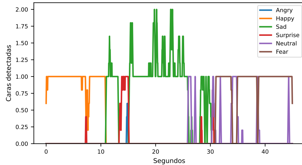
YOLOv8n imgsz=640 dets=1340 cov=94.9% 11.6 fps
