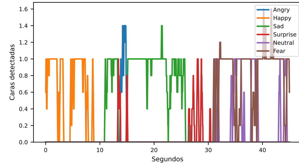
YOLOv11n imgsz=1280 dets=1088 cov=79.2% 2.4 fps
