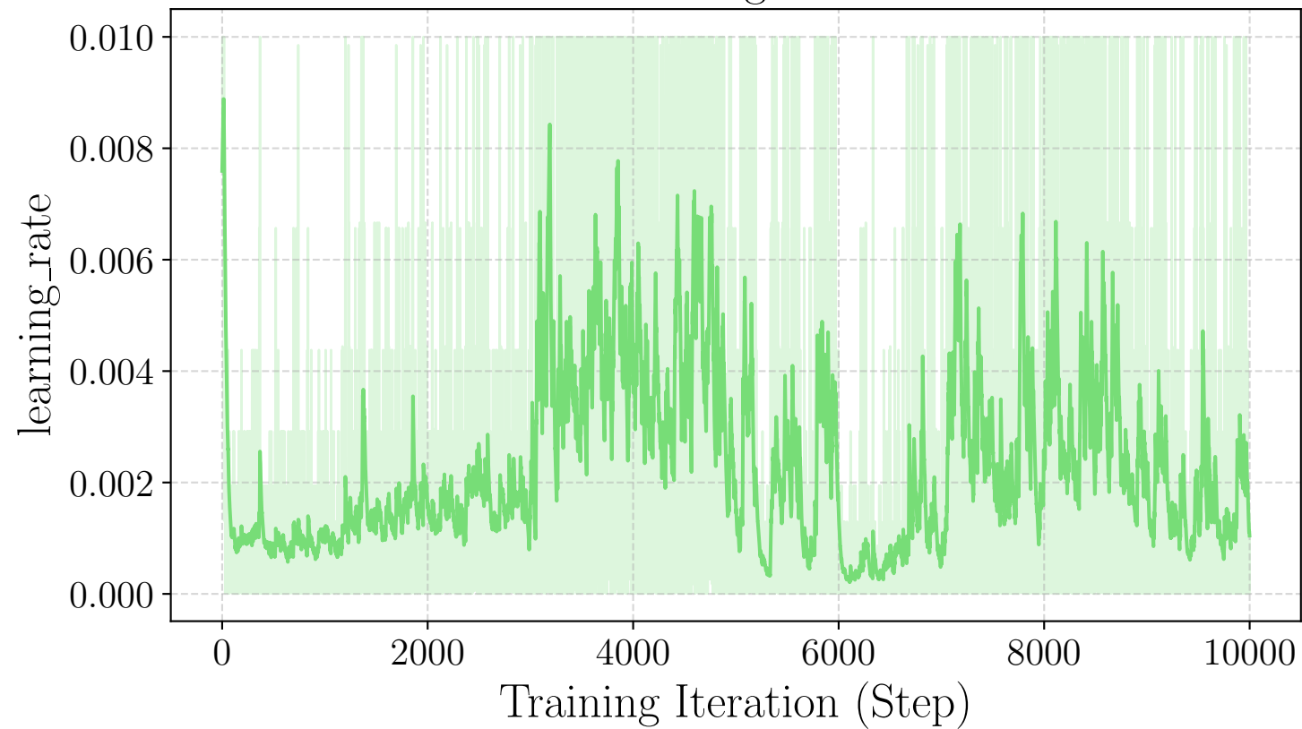
learning_rate
