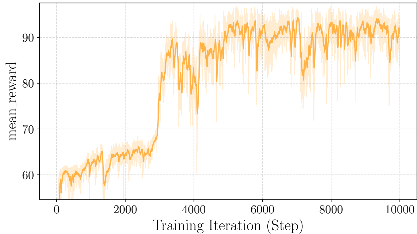
mean_reward
