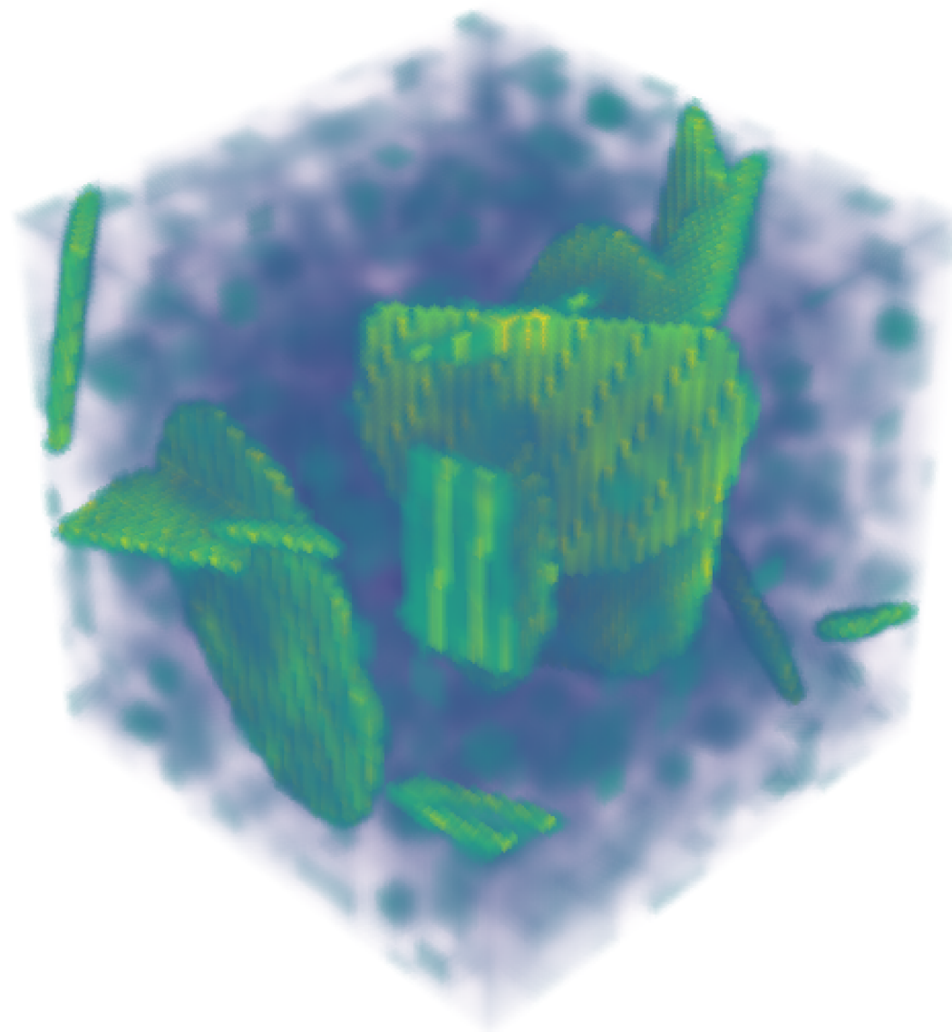
K_{xx} voxelized
