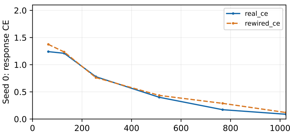
Validation learning curves: 32 fixed cases, distinct from the 128-case final test
