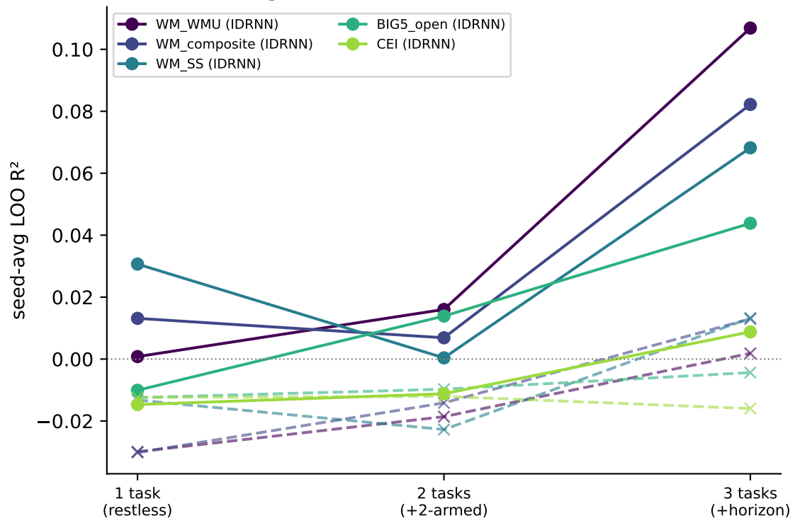
Per-target (solid=IDRNN, dashed=Vanilla)
