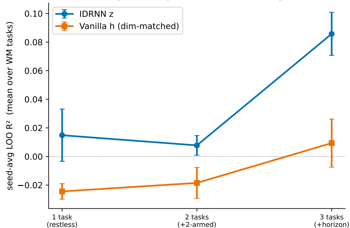
Working-memory readout vs training tasks
