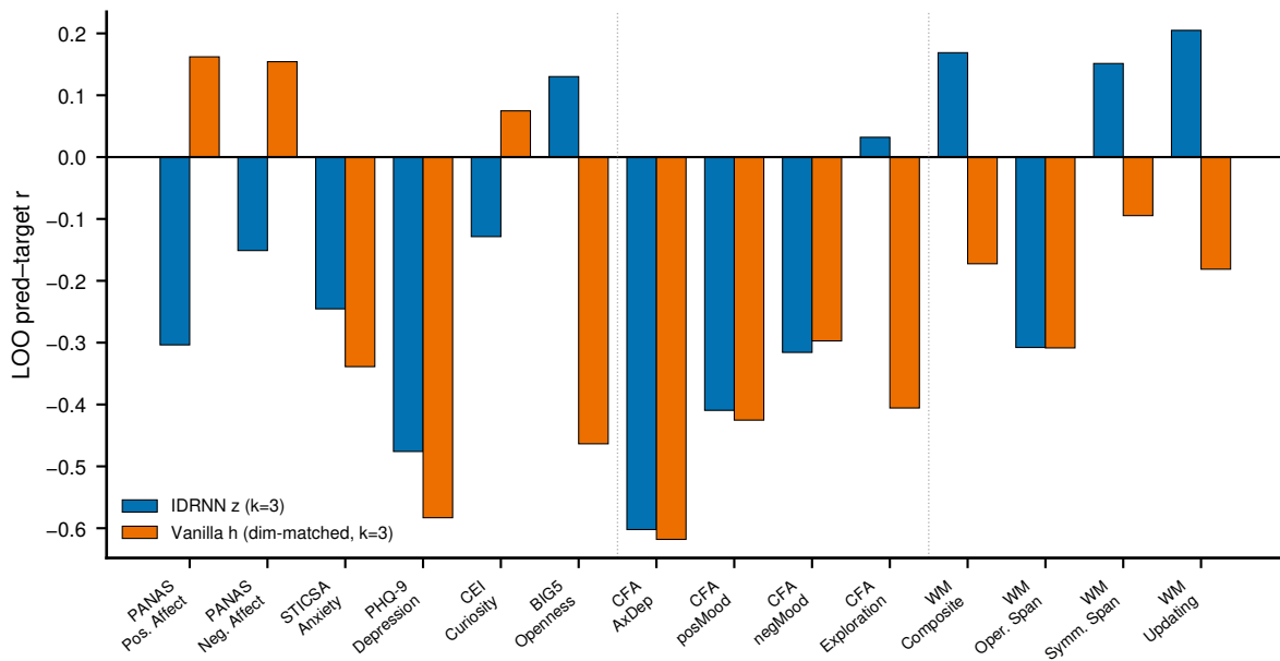
b LOO prediction–target r (neg = no-info artifact)
