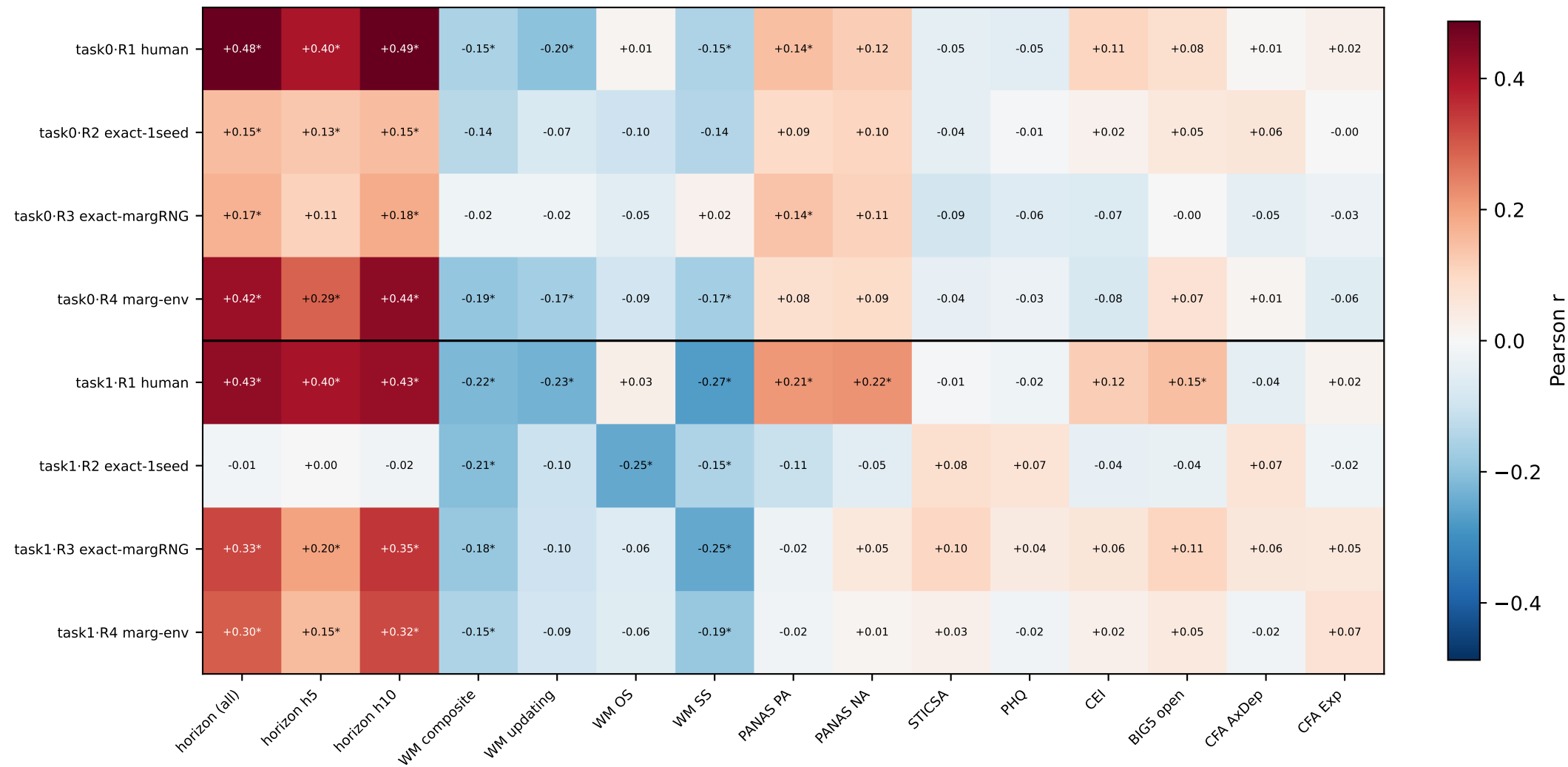
Regret → held-out target (Pearson r) [thalmann_z3_s2_full] top 4 rows = task0 predictor (noisier), bottom 4 = task1
