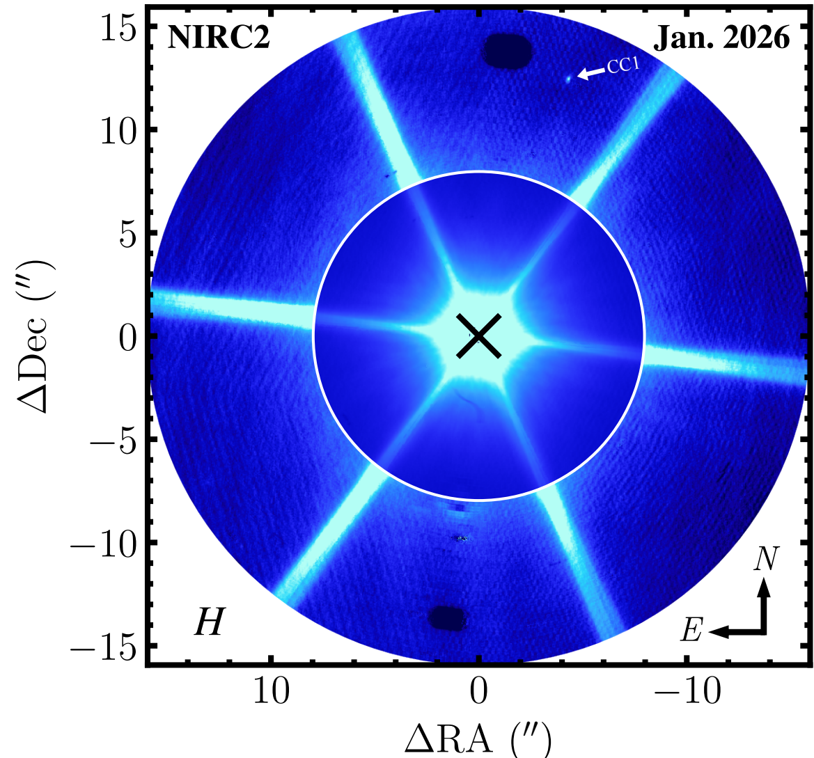
Keck / NIRC2 H Imaging
