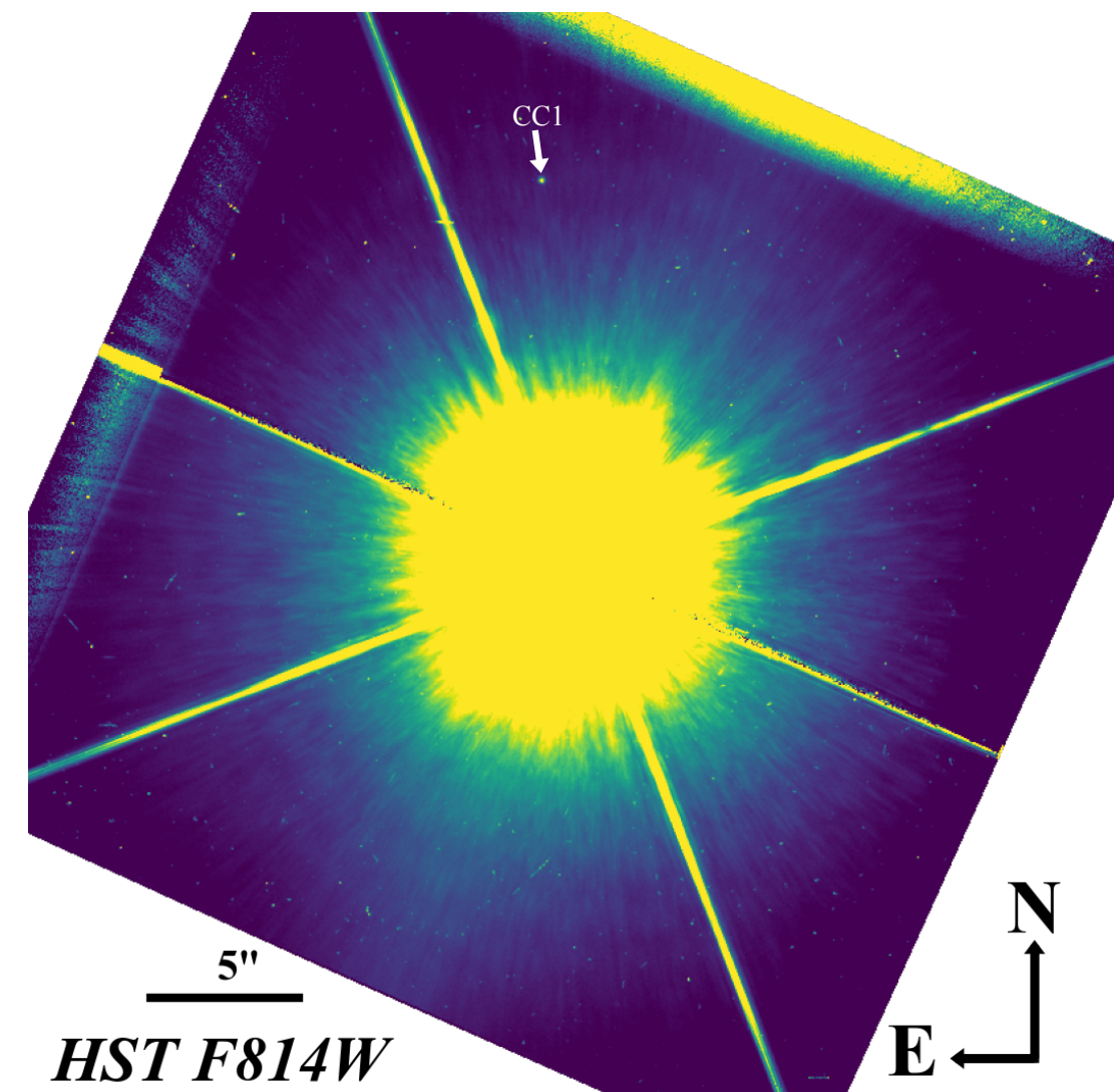
Hubble / WFPC2 Imaging
