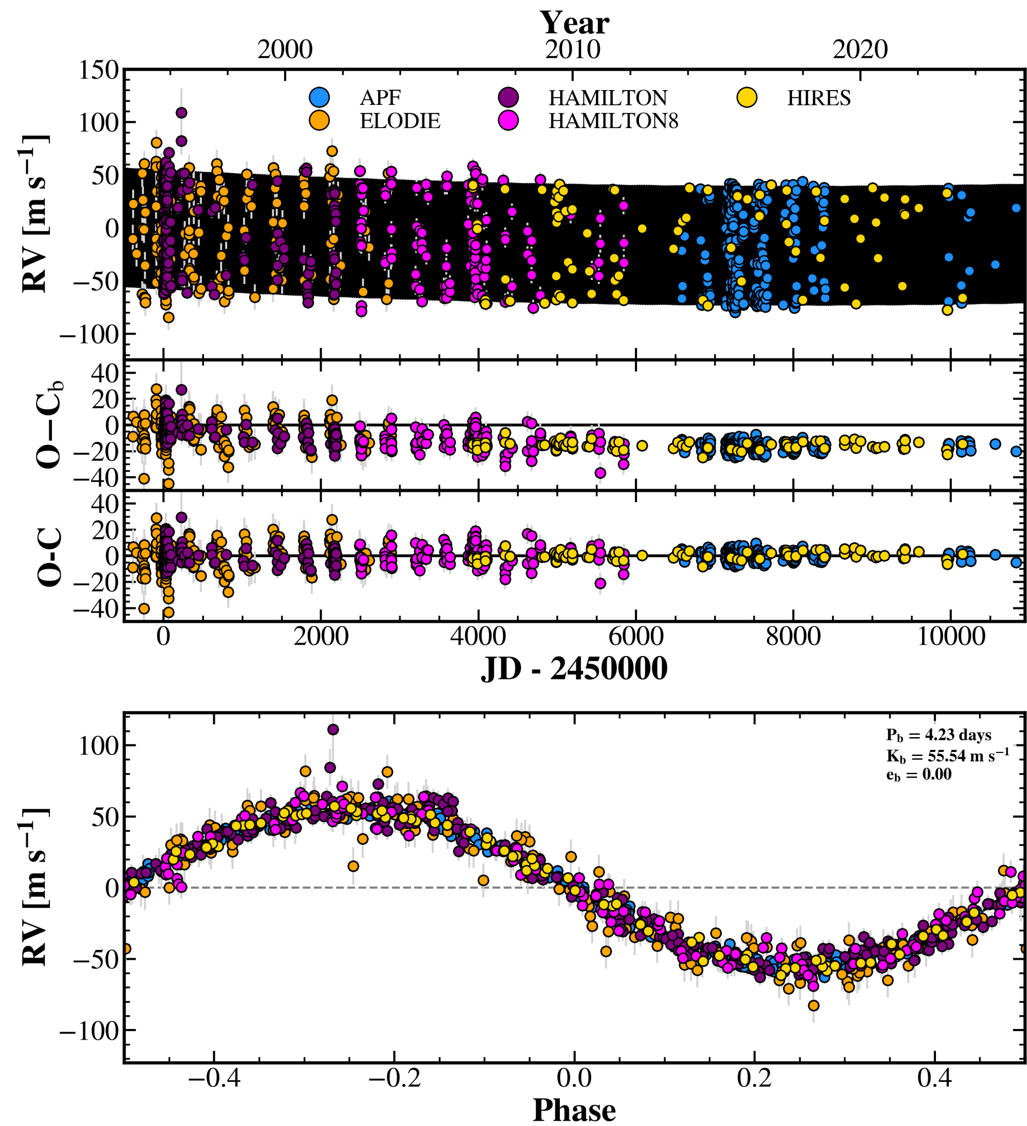
31 Year RV Baseline
