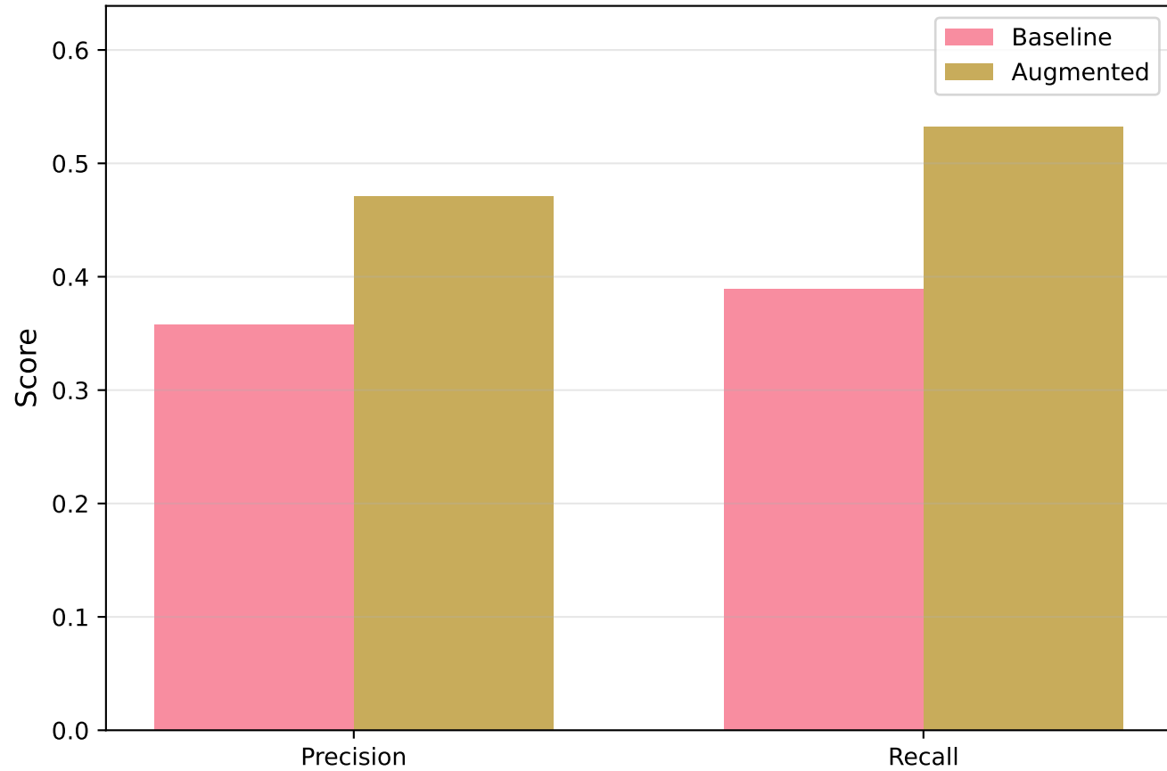
Test Set: Precision & Recall Comparison
