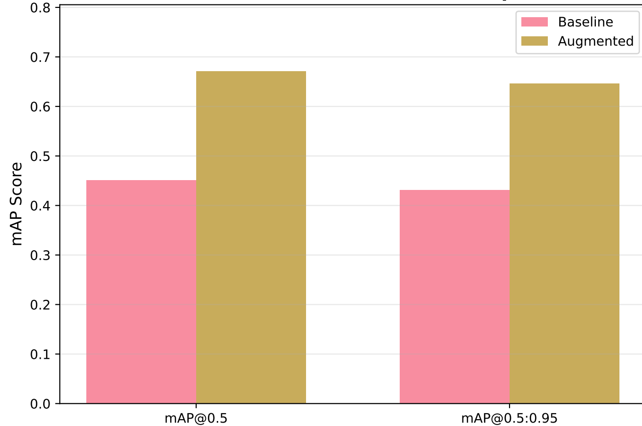
YOLOv8s Test Set: mAP Metrics Comparison
