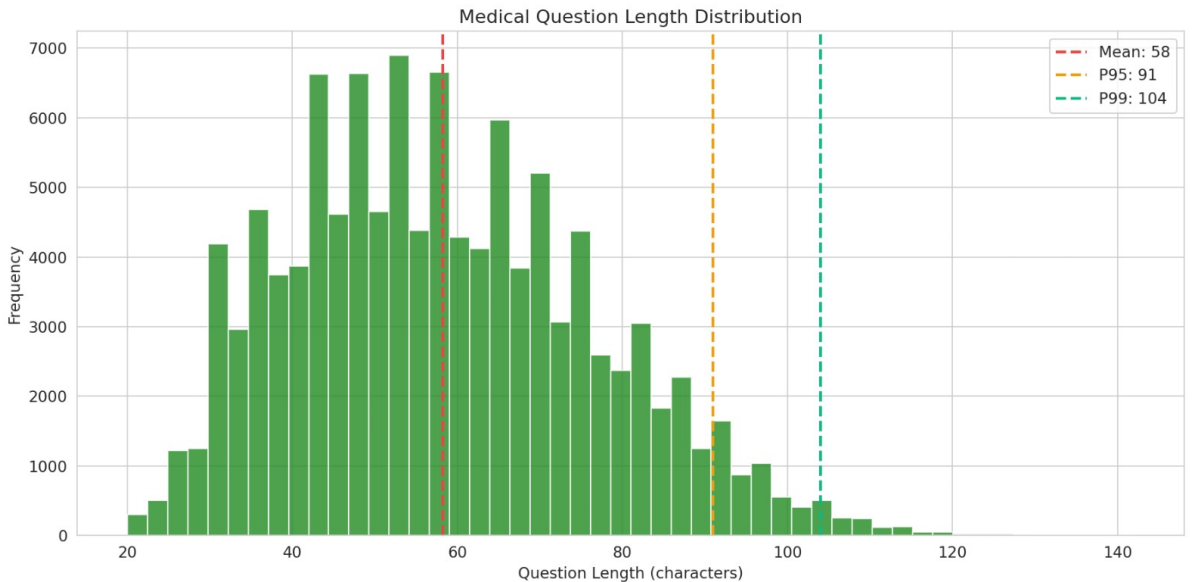
Figure 9: Distribution of Medical Question lengths after applying the 20-character minimum filter.
