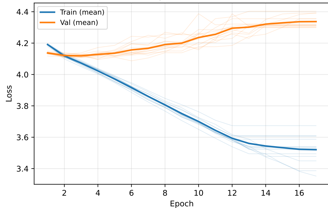
Stage 1 (InfoNCE)
