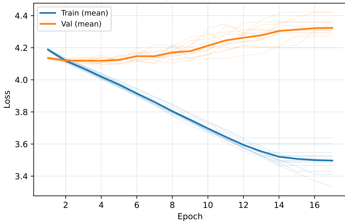
Stage 1 (InfoNCE)
