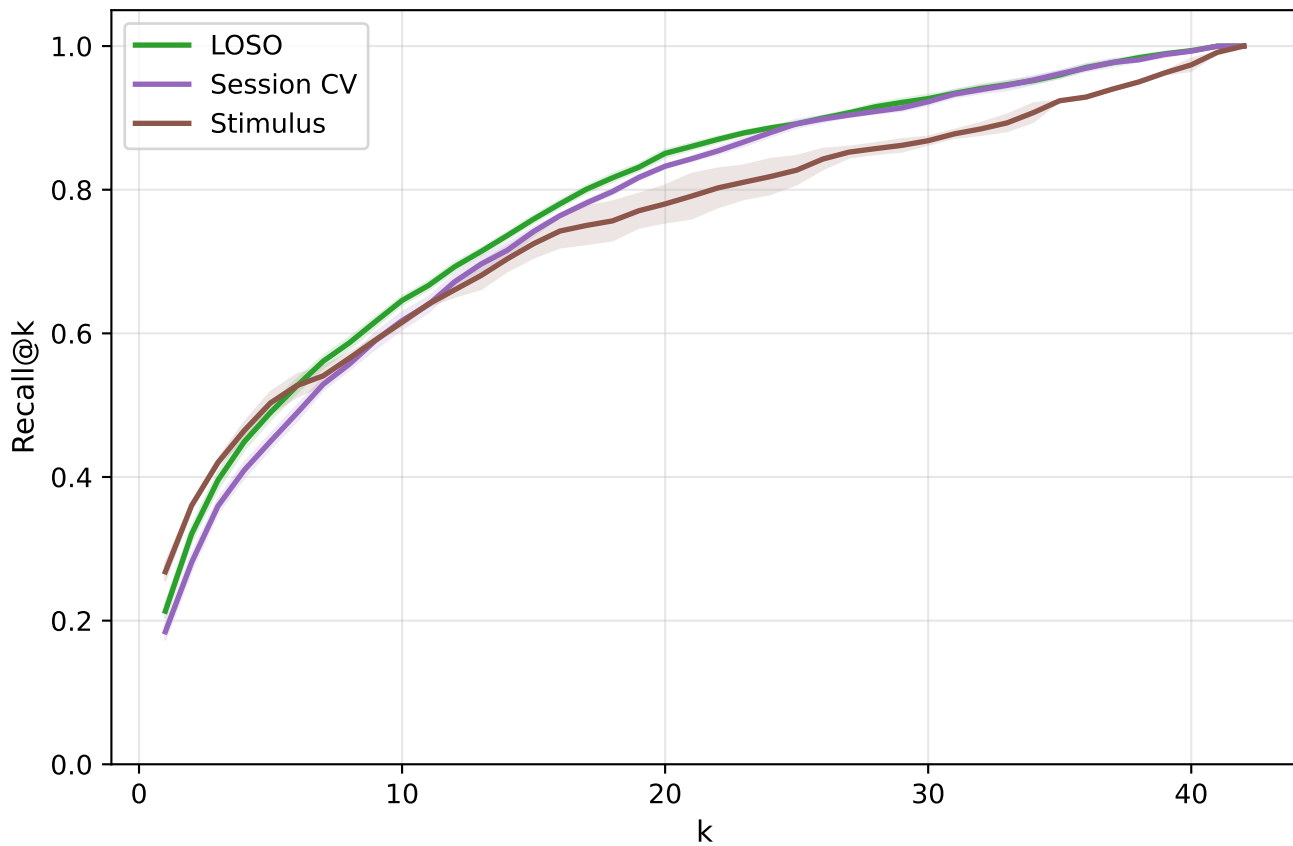
Recall@k — real condition across eval schemes (twostage)
