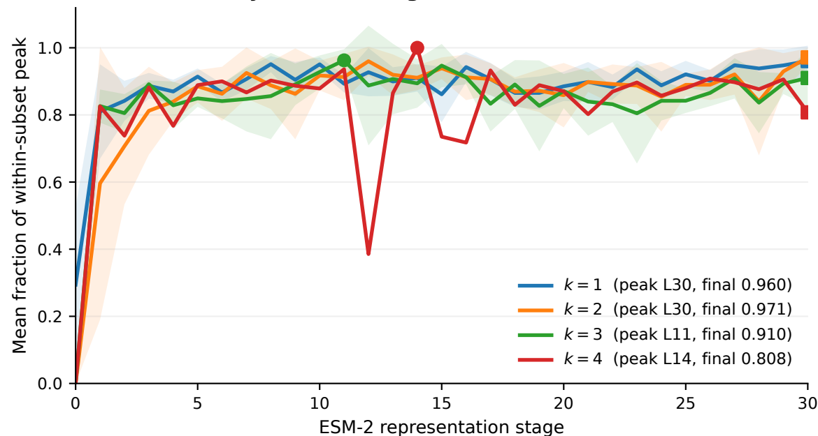
A Order-level dynamics through ESM-2
