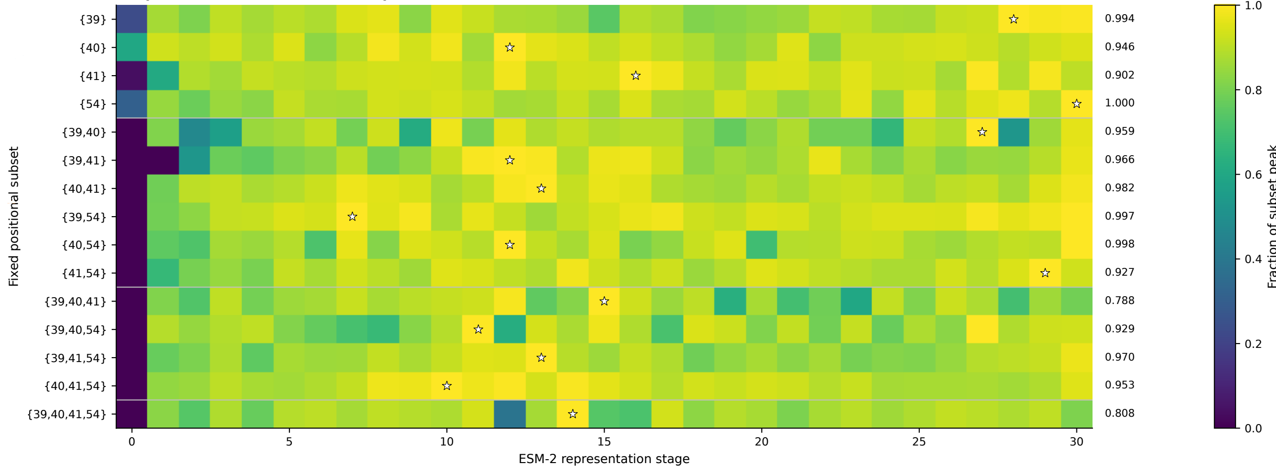
B Epistatic information transit map
