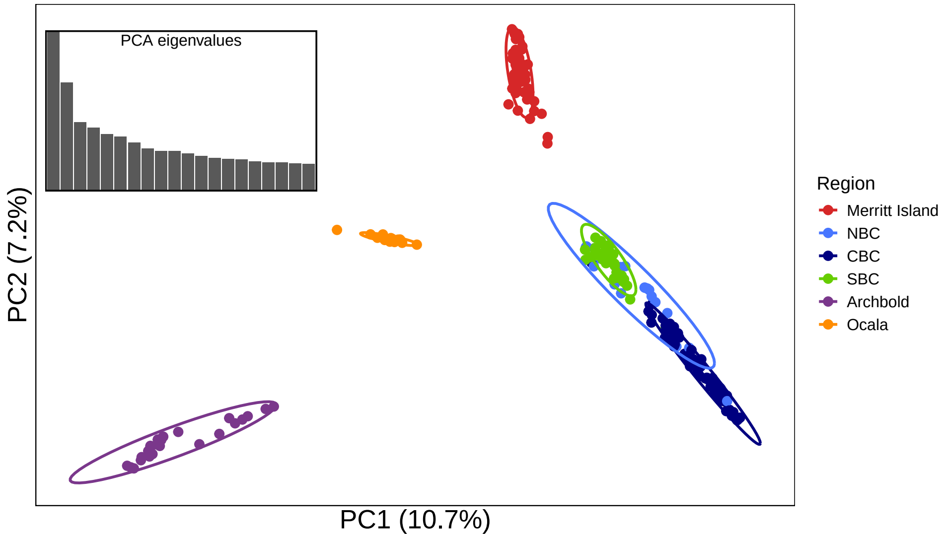
PCA of individuals across sampling regions
