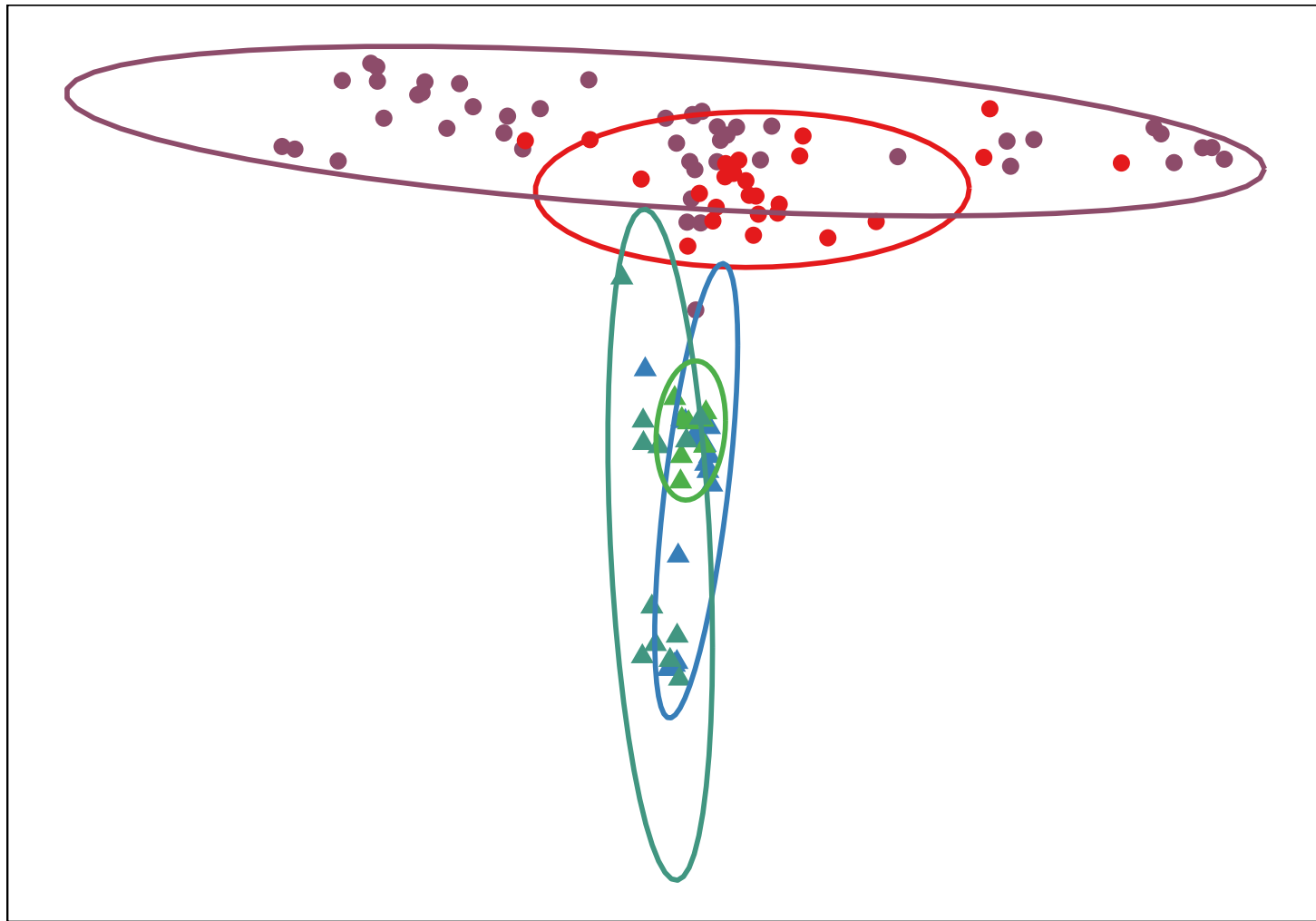
PCA of individuals across CBC and SBC
