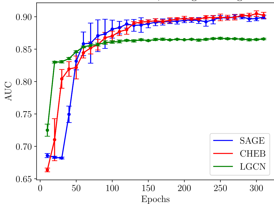
Amazon Data: AUC, 10 Negative Edges
