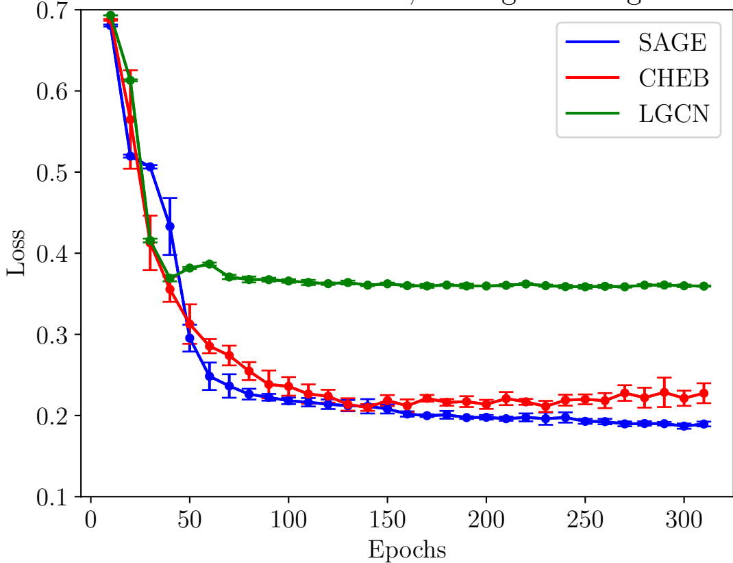
Amazon Data: Loss, 10 Negative Edges
