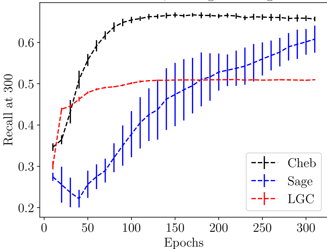
Recall at 300, 10 Negative Edges
