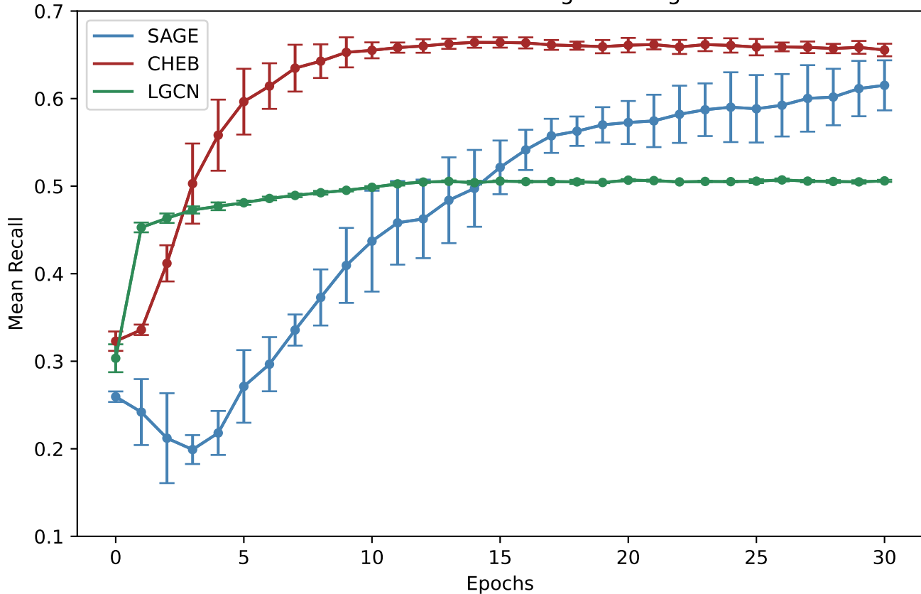
Mean Recall with 10 Negative Edges
