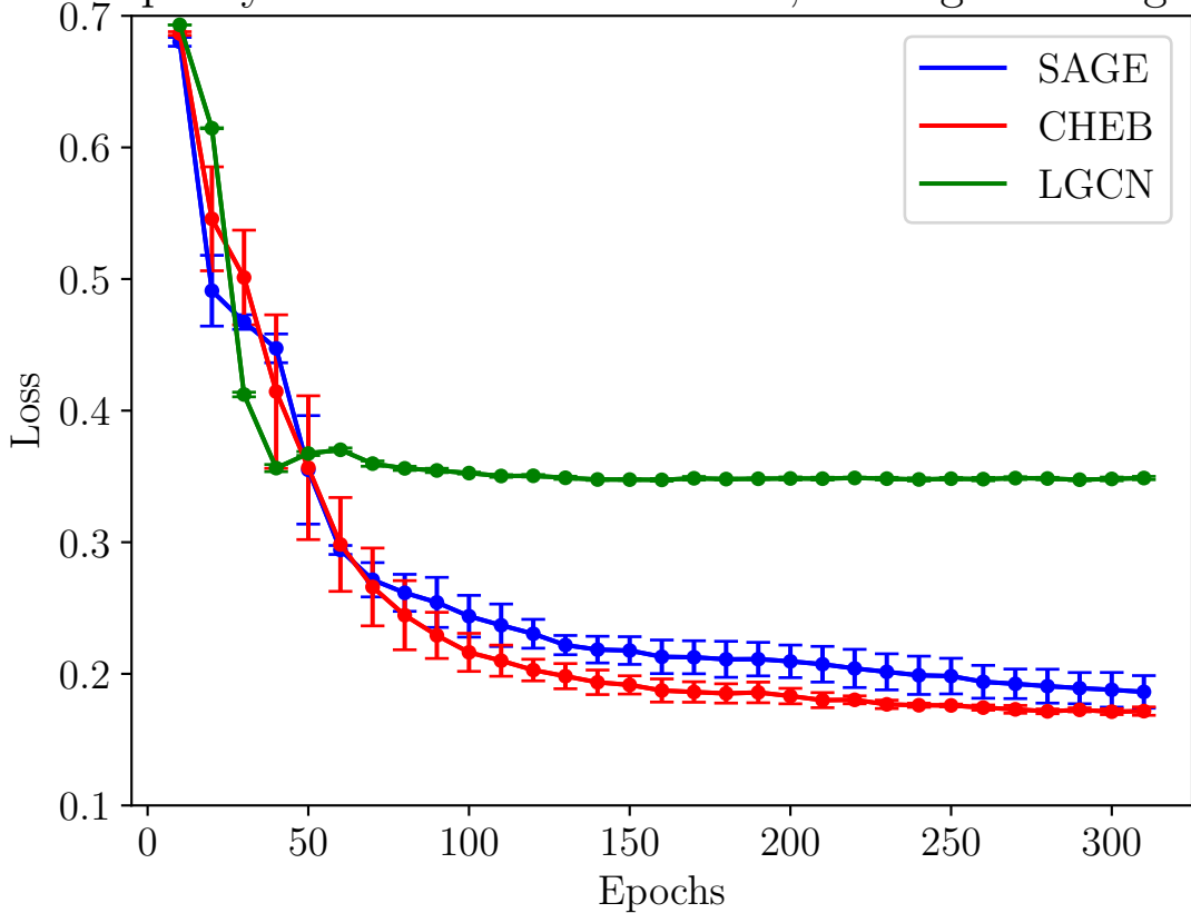
Spotify Data with Artists: Loss, 10 Negative Edges
