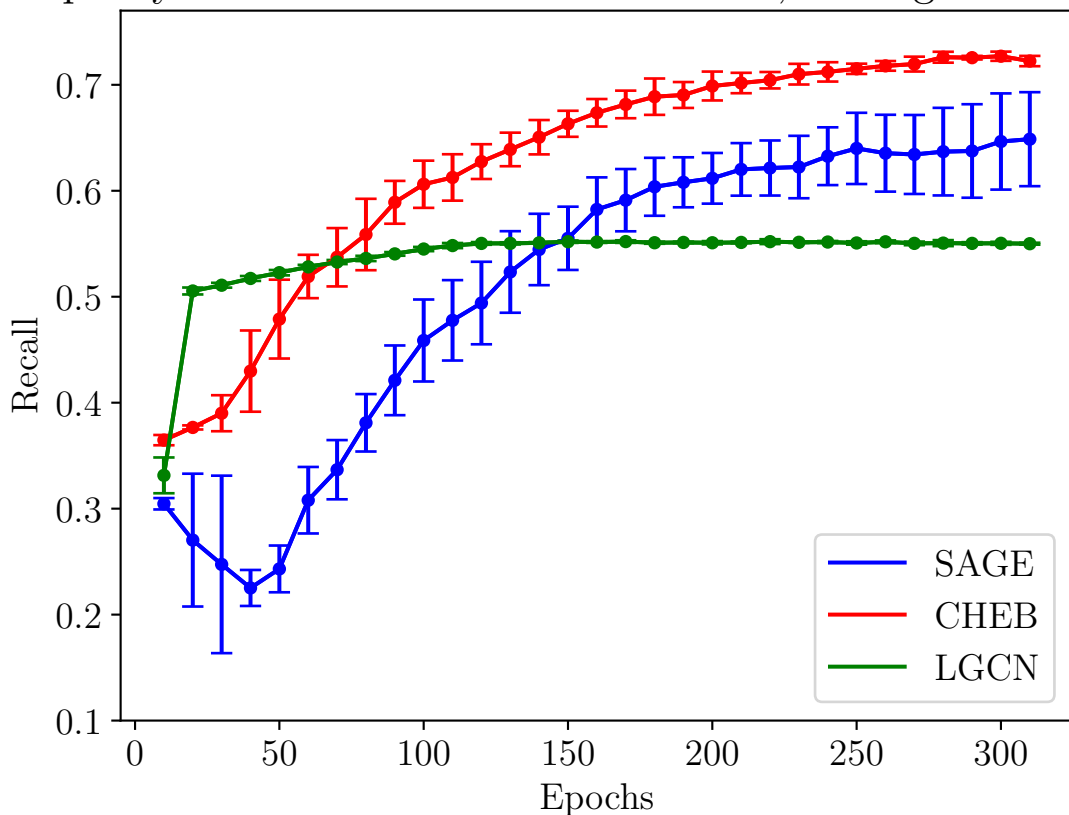
Spotify Data with Artists: Recall@300, 10 Negative Edges
