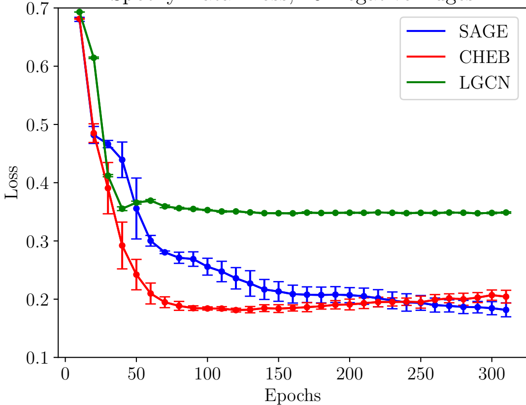
Spotify Data: Loss, 10 Negative Edges
