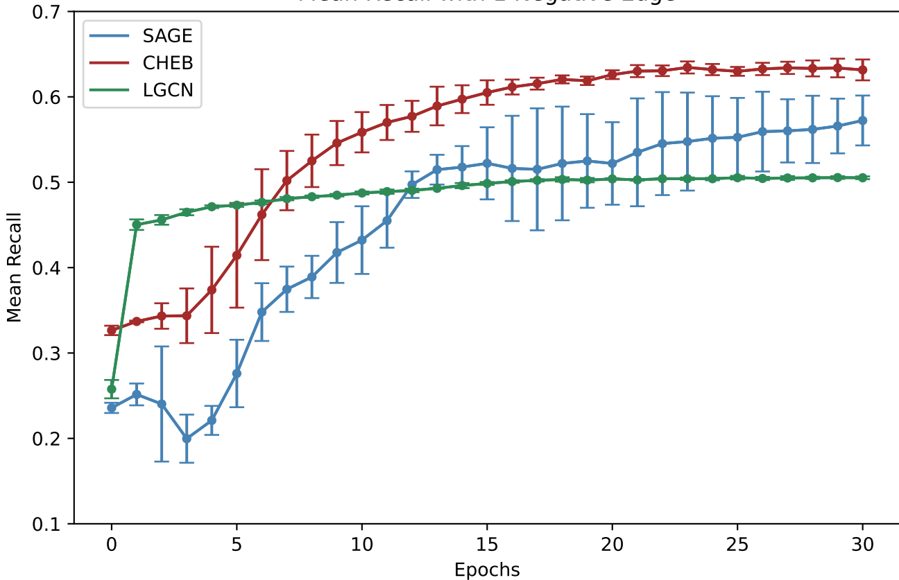
Mean Recall with 1 Negative Edge
