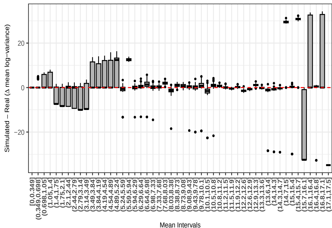
Figure 2: Distribution of the differences between simulated and real mean log-variance across 50 mean-abundance intervals, based on 100 simulations (AAM group).
