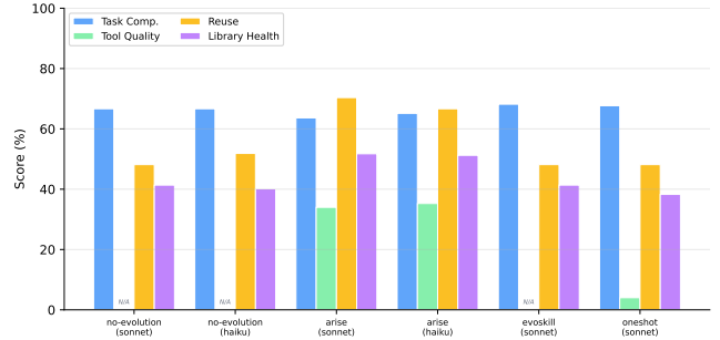
Figure 1: System comparison across four metrics (%). TC clusters all systems together (63–68%); library health separates them (38–52%). This illustrates the benchmark’s discriminative power beyond task completion.
