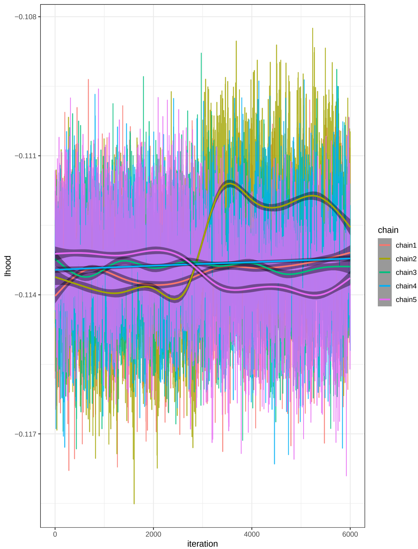
Likelihood trace plot
