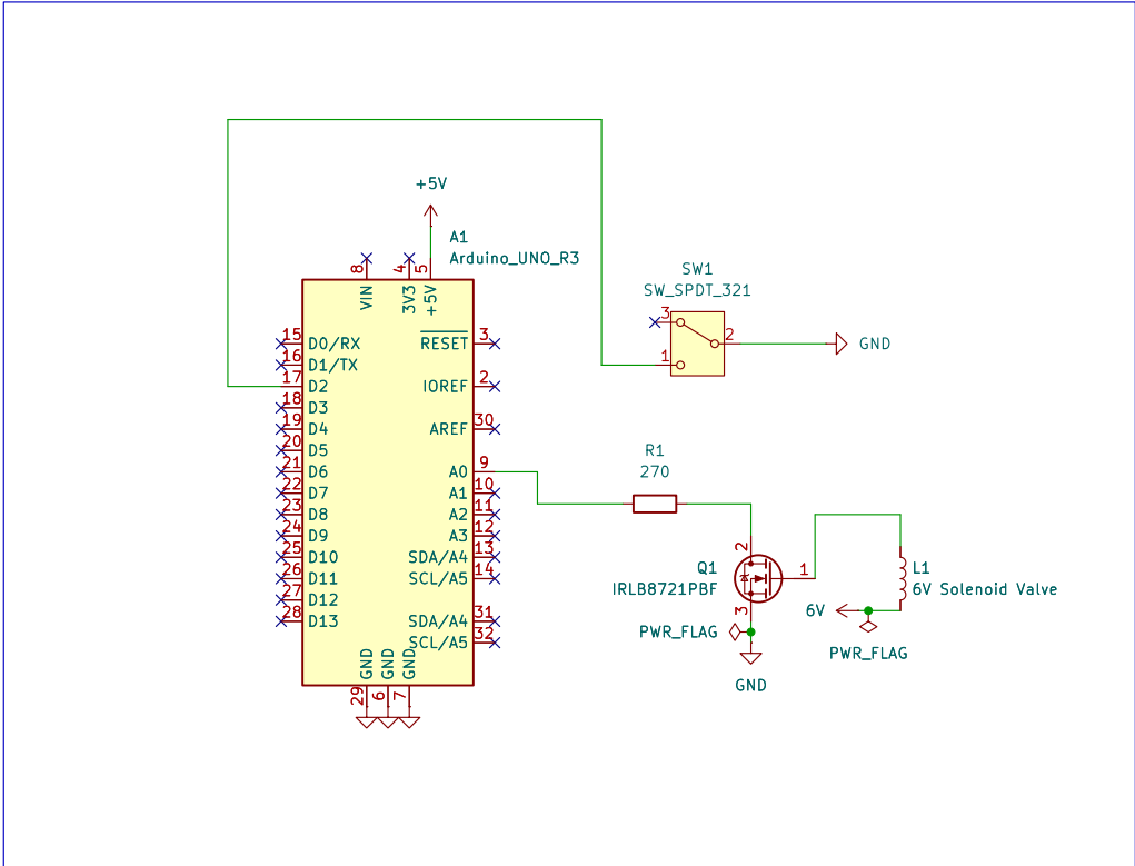
Microcontroller (Arduino UNO R3), 6V Solenoid Valve, Toggle Switch, N-Channel MOSFET
