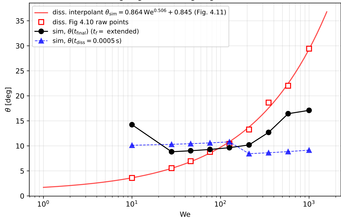
Receding angle vs leading-edge Weber number
