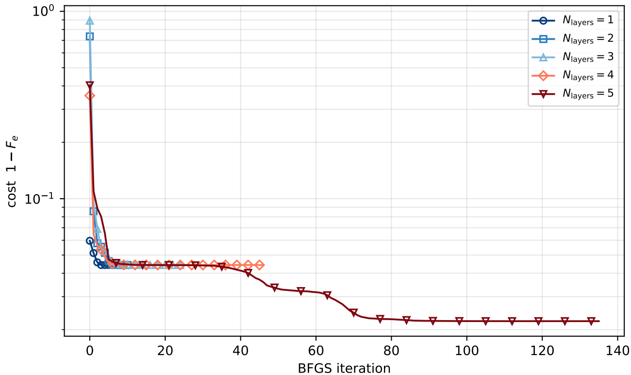
ECD+R compilation of TMS( r = 0.1 )
