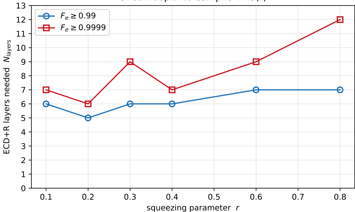
Circuit depth to compile TMS( r )
