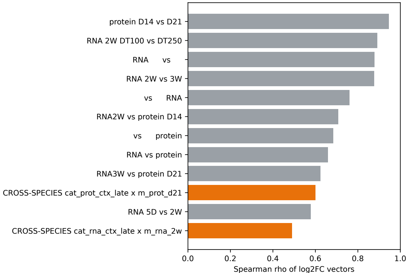
Cross-species similarity vs internal benchmarks
