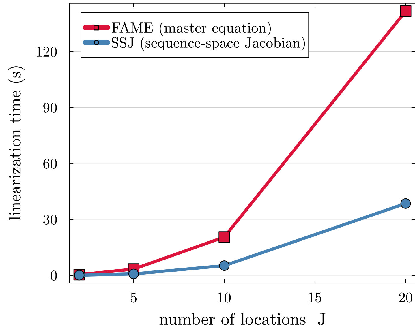
FAME vs SSJ: linearization time ( n = n_a \cdot J , n_a = 80 , T = 150 )
