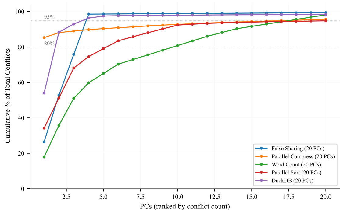
PC Conflict Concentration Across Benchmarks
