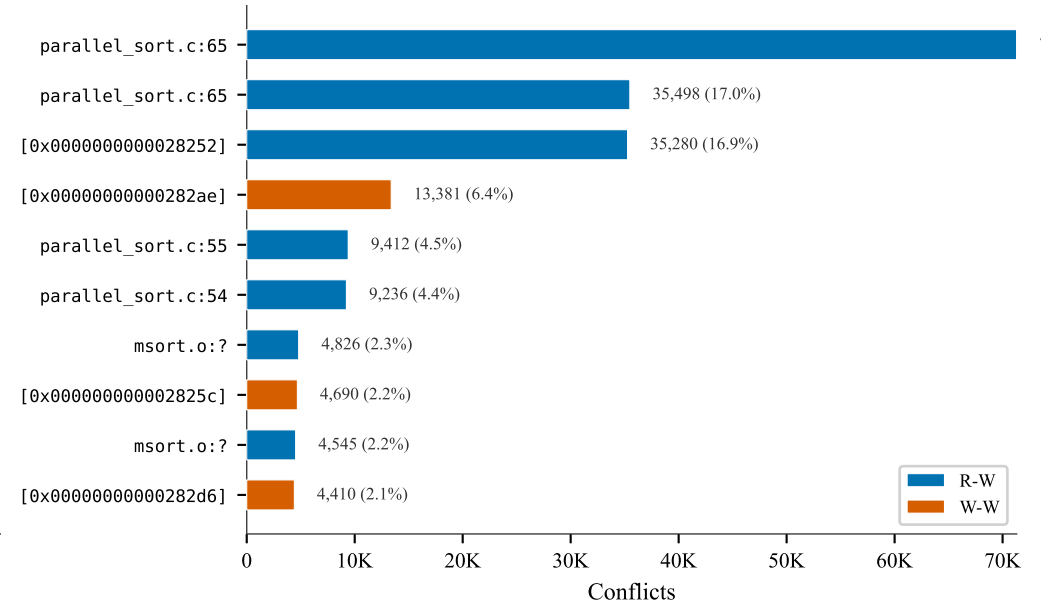
(b) Top-10 PC Hotspots
