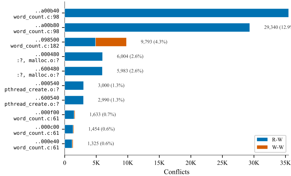
(a) Top-10 Contended Cache Lines
