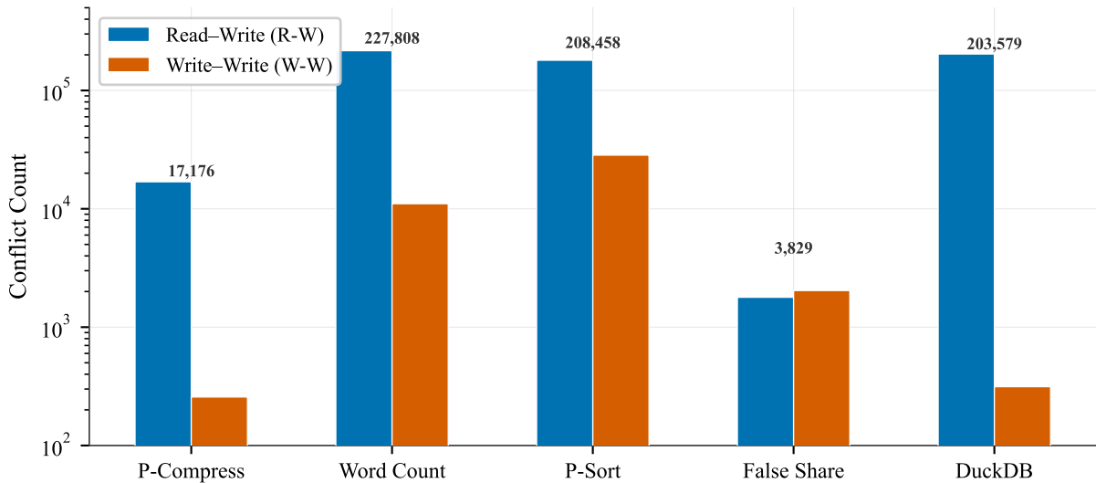
(a) Cross-Core Cache-Line Conflicts by Benchmark
