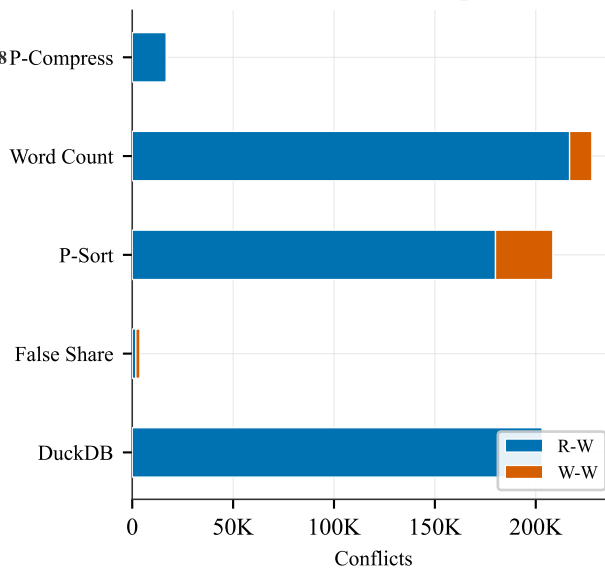
(b) R-W vs W-W Split
