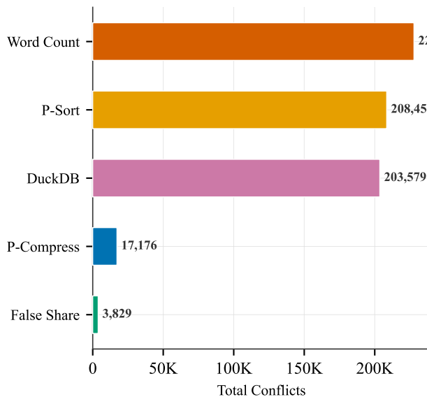
(a) Total Conflicts
