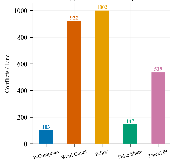
(f) Conflict Intensity
