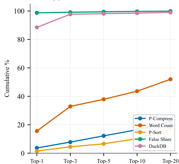
(e) Cache-Line Concentration
