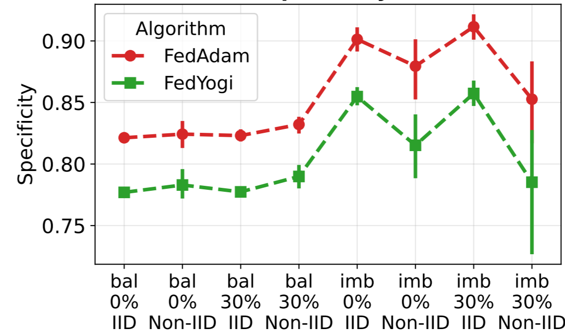
Specificity
