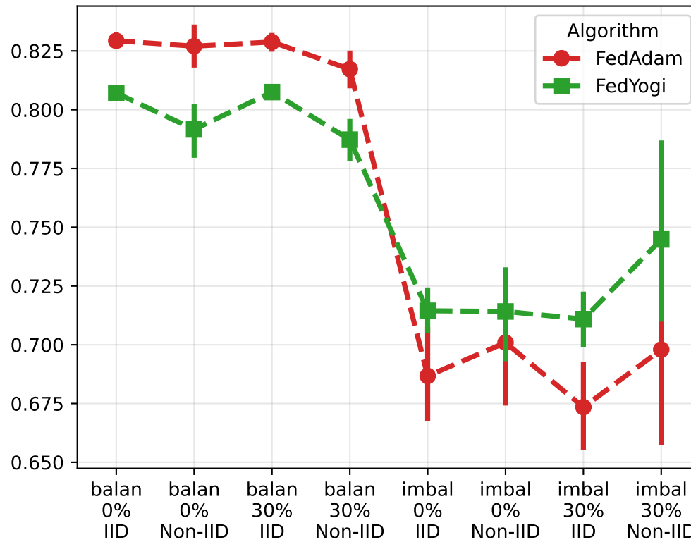
Recall
