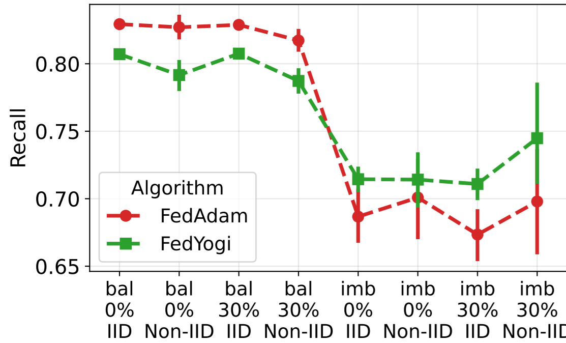
Recall
