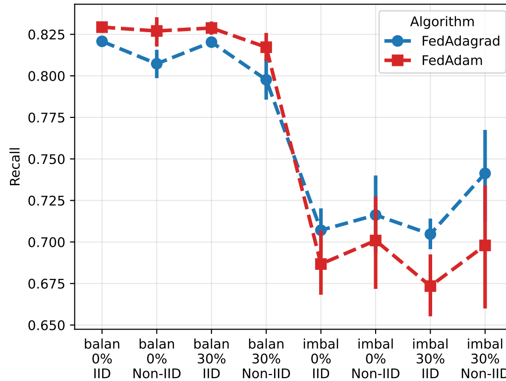
Recall
