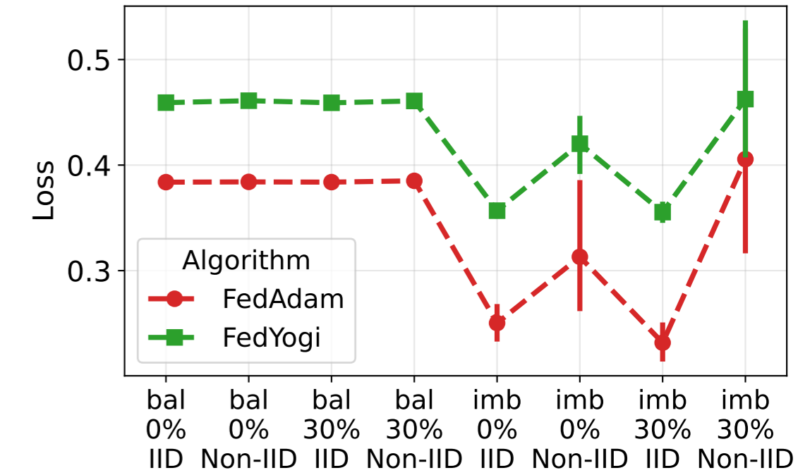
Loss
