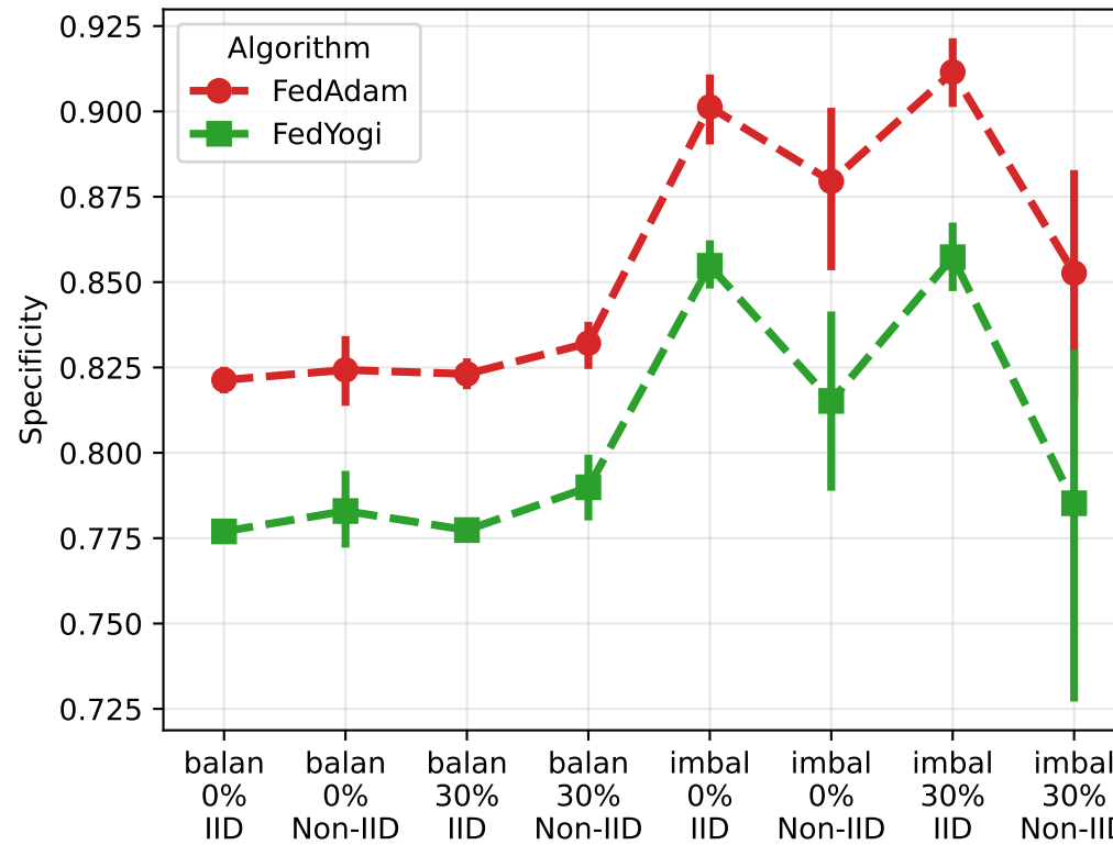
Specificity
