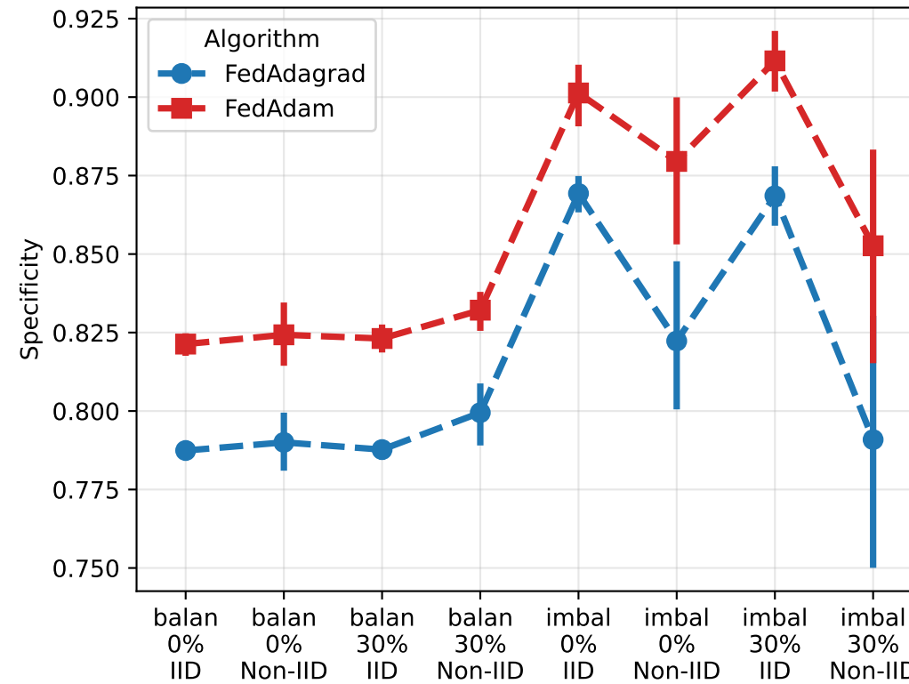
Specificity
