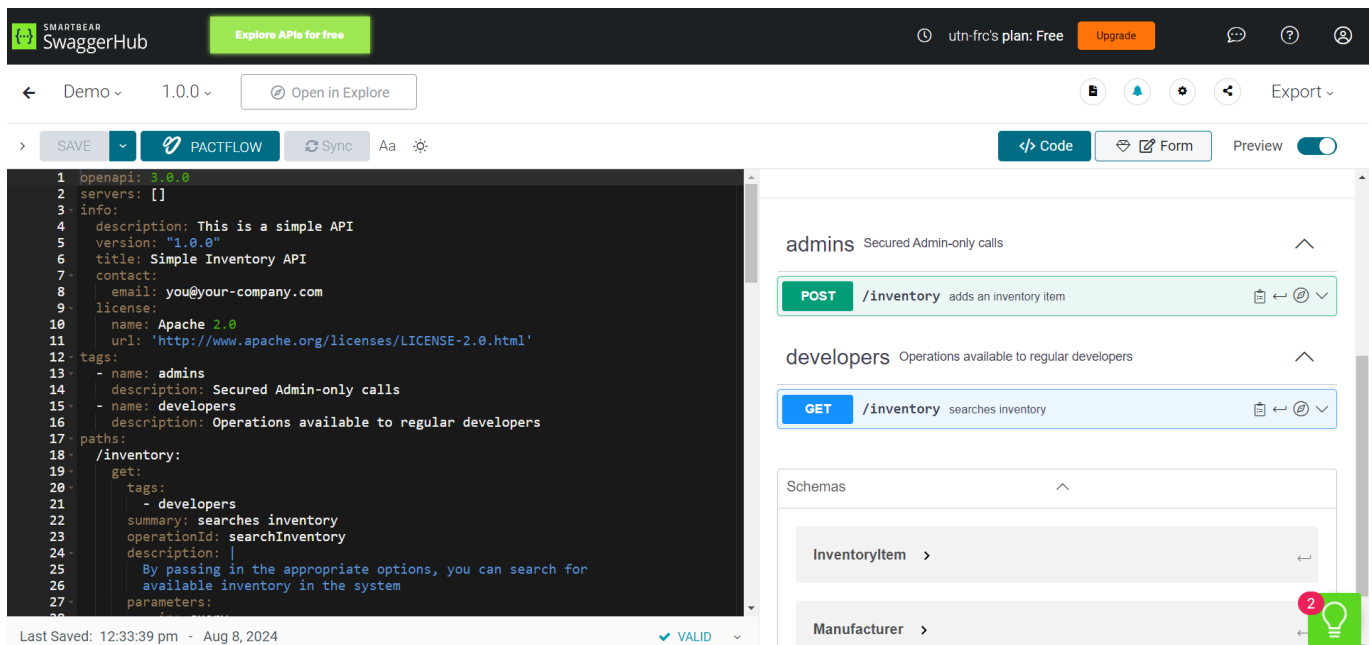
Figura 5: SwaggerUI designer
