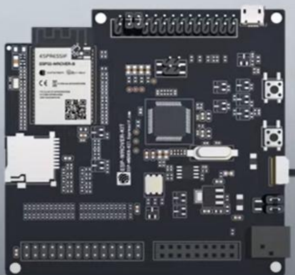
ESP32-WROVER-KIT-VB
