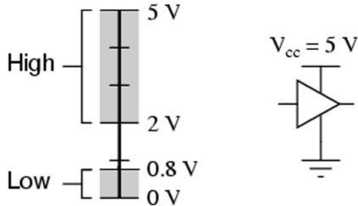
Acceptable TTL gate input signal levels
