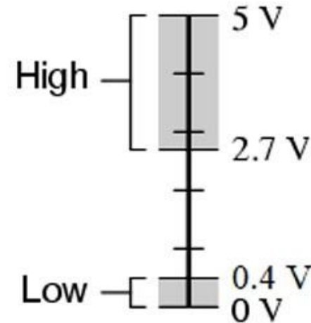
Acceptable TTL gate output signal levels
