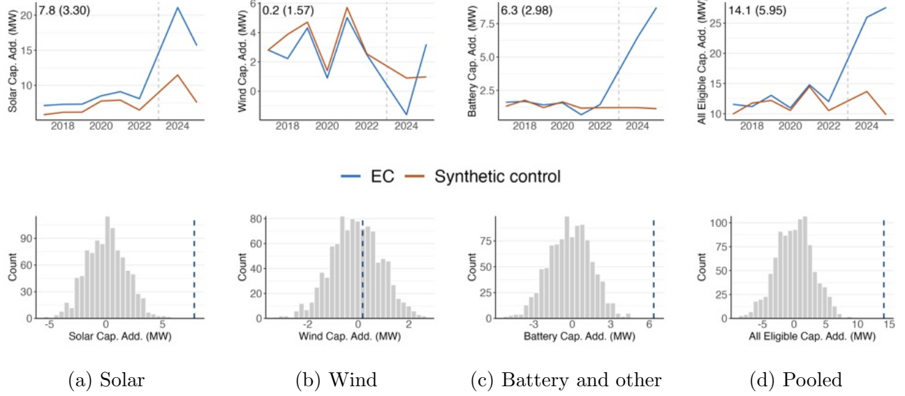
Figure 5: Capacity addition SDID and permutation test results. Pooled treatment effects reported at the top, with bootstrapped standard errors in parentheses. EC stands for Energy Community.
