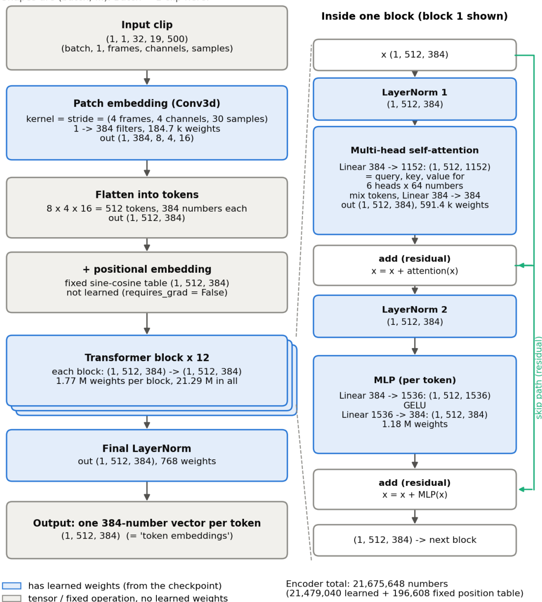
Figure 3: EEG-VJEPa's Vision Transformer — patch and tubelet sizes, the resulting 512-token × 384-number grid, and the stack of self-attention blocks that process it [1].
