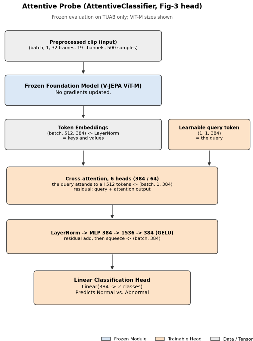
Figure 15: The paper’s Fig-3 Attentive Probe — a learnable query token attends over all 512 tokens via full multi-head cross-attention, followed by an MLP [1].
