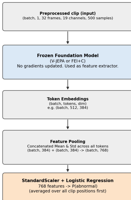
Figure 13: The Linear Probe — mean and standard deviation pooled over all tokens (or, for FEI/GTJ, the raw embedding), then a StandardScaler + logistic regression.
