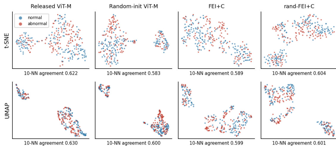
Figure 18: t-SNE (top) and UMAP (bottom) maps of four feature sets on TUAB — blue = normal, red = abnormal. No map, learned or random, shows the two labels forming separate regions.
