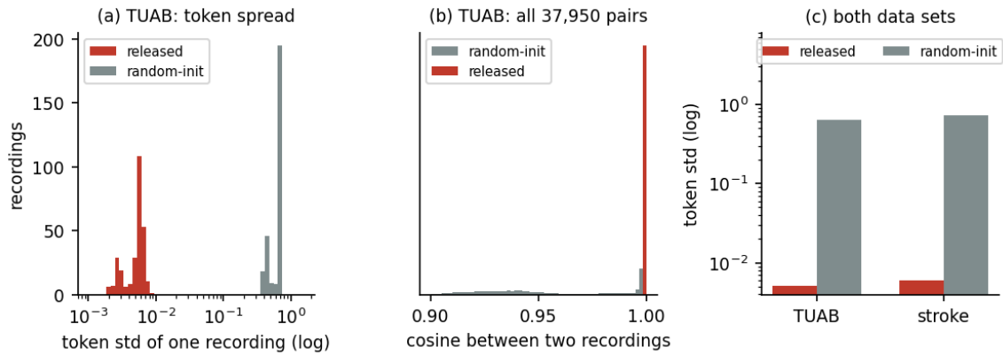
Figure 16: Direct evidence of representation collapse — the released checkpoint's per-recording output spread (token std) is about 125\times smaller than a random-weight twin's, on both TUAB and the (never-seen-in-pretraining) stroke dataset, and its recordings are almost perfectly cosine-similar to one another (mean 0.999982) regardless of diagnosis. Token spread is the deciding measure; random weights also reach a cosine of 0.9991 on the stroke cohort.
