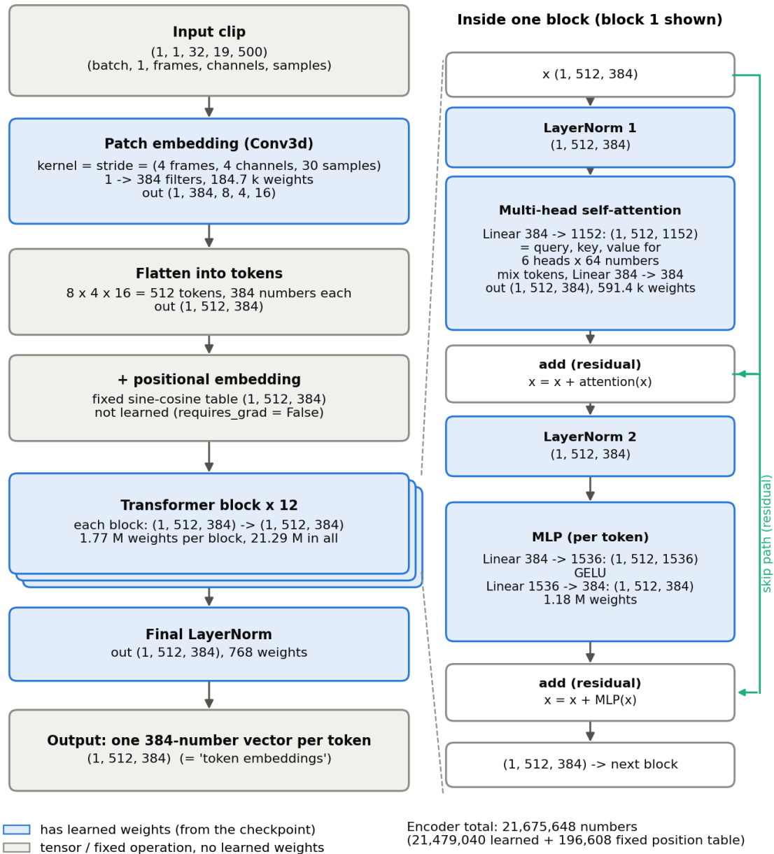
Figure 3: The Vision Transformer of EEG-VJEPa: patch and tubelet size, the resulting 512-token \times 384-number grid, and the stack of self-attention blocks that process this grid [1].
