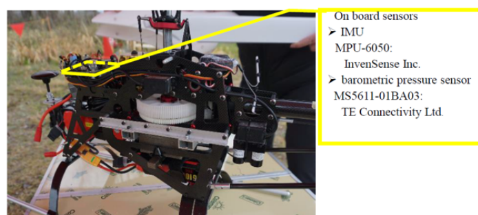
Fig.2.4: IMU(Inertial Measurement Unit)
