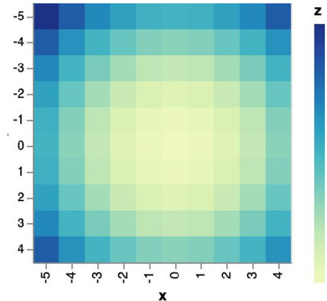
Heatmap
